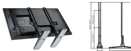
Foot Stand SBM-320ST
